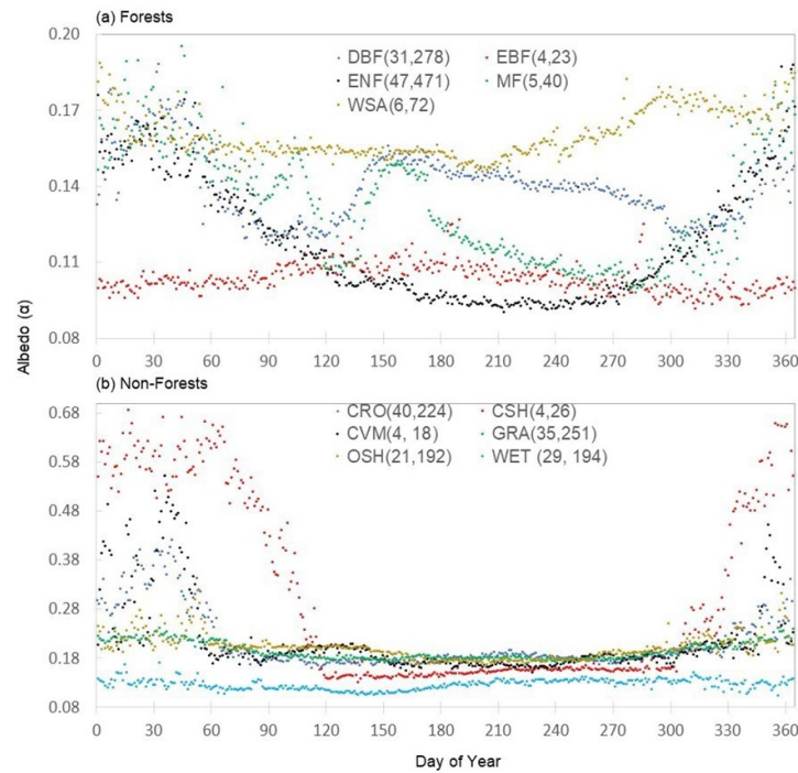
Figure 2. (a) Daily time series of midday albedo (11:00–13:00 h local time) were analyzed from selected AmeriFlux sites (SI-2), grouped as forest clusters based on IGBP land cover classifications. Each time series represents a composite of data from all available years and sites. (b) Daily time series of midday albedo (11:00–13:00 h local time) for non-forests. Each time series represents a composite of data from all available site and site-year. The first numbers in parentheses indicates the total number of sites used for calculating the average albedo values, and the second number indicates the total site-year used for each type. Cover types with less than 4 tower sites are excluded.
