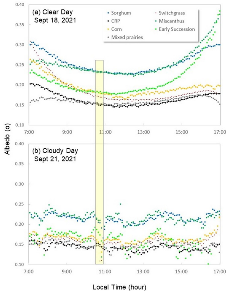
Figure 3. Diurnal changes and variations in land surface albedo under clear (a) and cloudy (b) sky conditions for seven bioenergy crops at the Kellogg Biological Station (KBS) in Southwest Michigan, USA. The yellow shaded area on the bar graph represents the local time ( \sim 10:30 h) when the Landsat/Terra satellites pass over the study sites.
